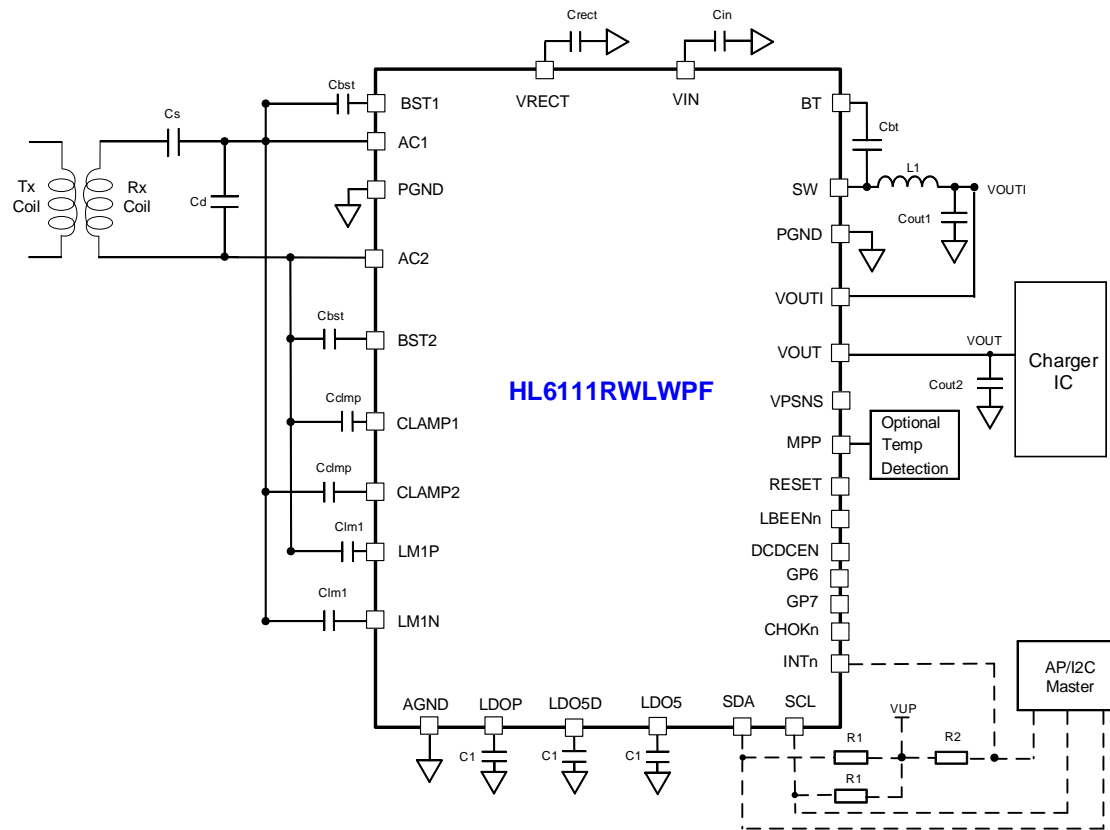
Figure 1 HL6111RWLWPF Typical Application and Functional Diagram
